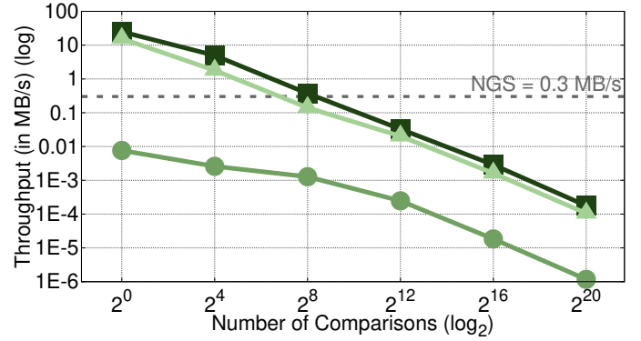
Figure 5. Average throughput of GenoDedup writes with different indexes for QS using a single thread.
