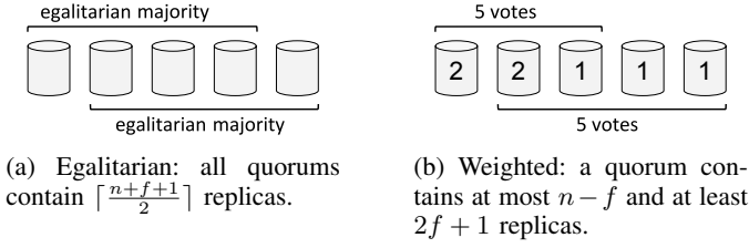
Figure 2: Possible quorums for n = 5 , f = 1 , \Delta = 1 (BFT).
