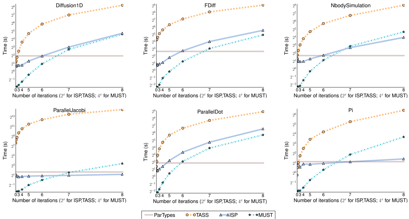
Figure 11. Results for the experiments varying the number of loop iterations
