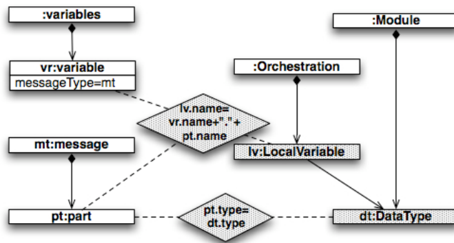
Fig. 6. Transformation rule for variables declaration. A BPEL variable refers to a message composed by parts. A local variable is created, for each part of each BPEL variable, in the orchestration of the business role typing the central component that is the only orchestration in the module
