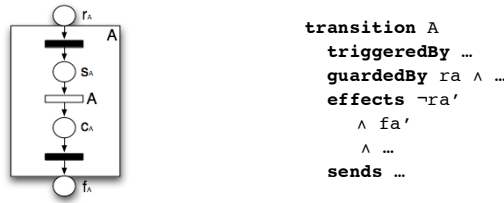
Fig. 5. A simplified version the Petri Net representation of a generic BPEL activity A [12], and the corresponding SRML transition. Additional statements have to be added to model the execution of the activity.
