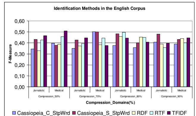
Figure 7. Text clustering values in the Corpus in English with internal measure using the harmonic FMeasure.
