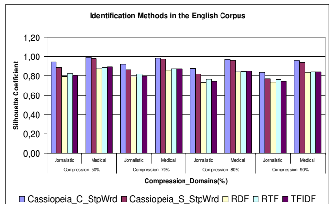
Figure 11. Text clustering values in the Corpus in English with external measure using the harmonic Silhouette Coefficient.
