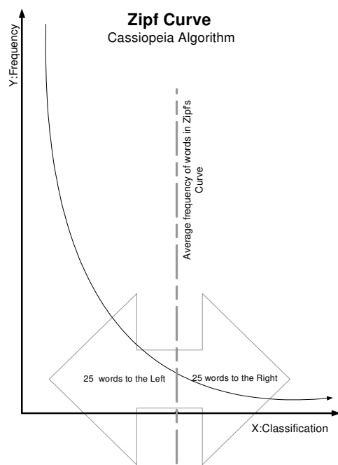
Figure 2. Selection of Attribute in the Cassiopeia model.
