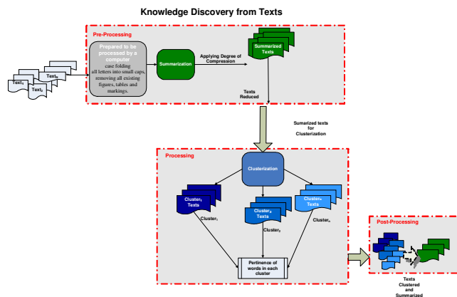
Figure 1. The Cassiopeia Model.
