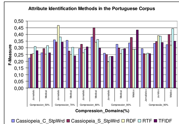
Figure 3. Text clustering values in the Corpus in Portuguese with internal measure using the harmonic FMeasure.
