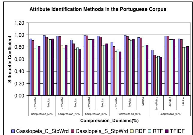
Figure 10. Text clustering values in the Corpus in Portuguese with external measure using the harmonic Silhouette Coefficient.
