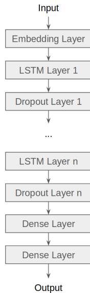
Fig. 6: High level view of our model.
